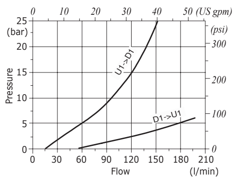
VODL/SC 100 pressure drop vs. flow from D1->U1 and U1->D1
