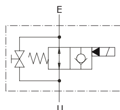
Normally closed configuration (NA)
