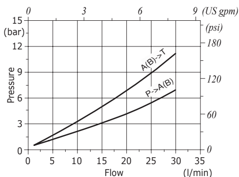
VIA/AP 6-38 pressure drop vs. flow
