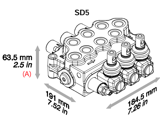
(A) quota riferita sul piano utilizzi (A) dimension is referred to working ports surface
