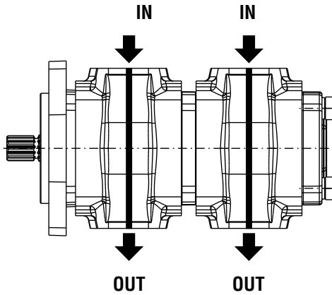
STANDARD VERSION
