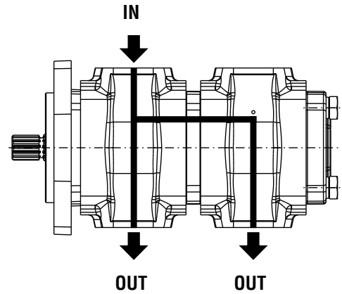
COMMON INLET
